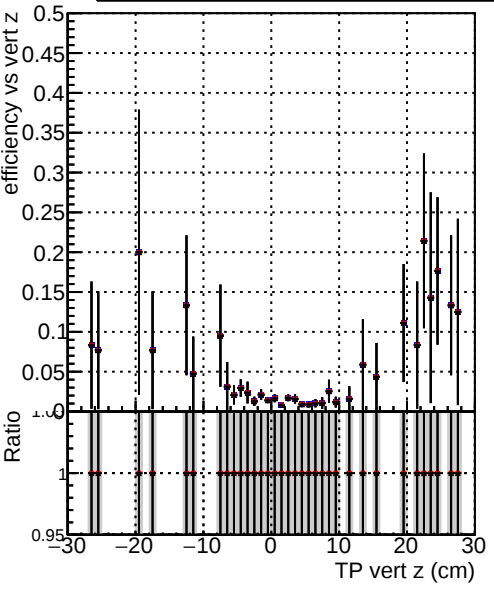
Efficiency vs vertpos Legend: DQM_TT_originalREDO100 DQM_TT_originalREDO100f DQM_TT_originalREDO100fb
