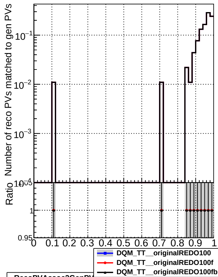
RecoPVAssoc2GenPVMatched_missing
