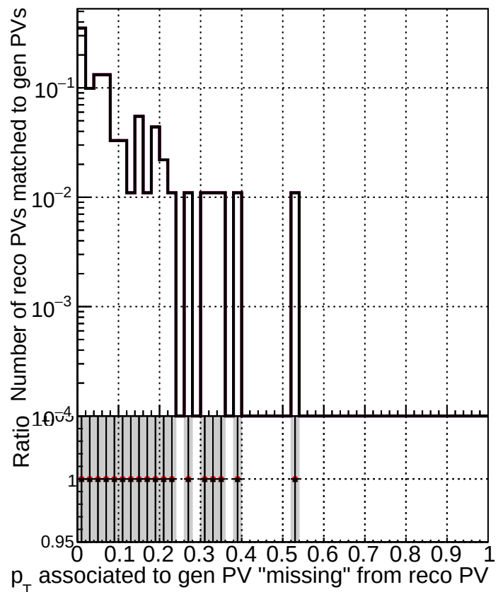
RecoPVAssoc2GenPVMatched_missing
