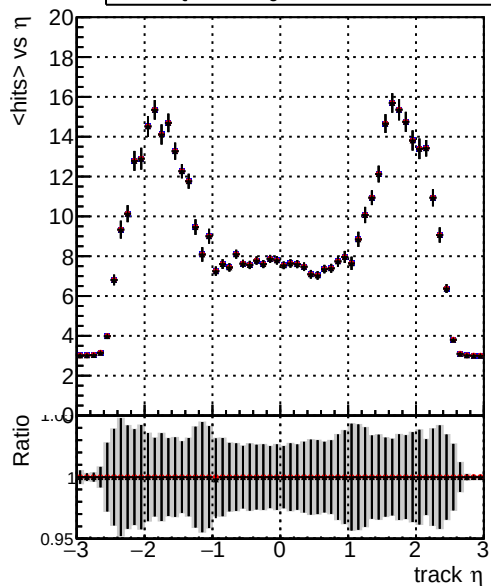
mean hits DQM_TT_originalREDO100f DQM_TT_originalREDO100f DQM_TT_originalREDO100fb
