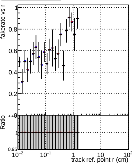
Legend: - blue dots: DQM TT originalREDO100 - red dots: DQM TT originalREDO100f - black dots: DQM TT originalREDO100fb
