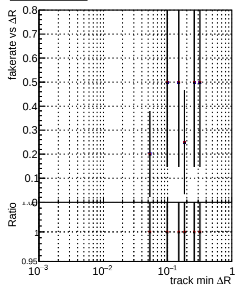
Fake rate vs \Delta R(\text{track, jet}) Legend: DQM TT originalREDO100 (black line) DQM TT originalREDO100f (red line) DQM TT originalREDO100f (blue line)
