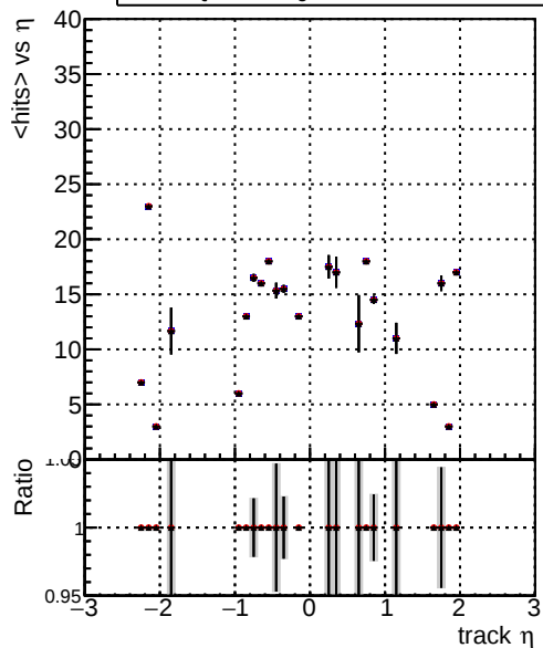
mean hit DQM_TT_originalREDO100 DQM_TT_originalREDO100f DQM_TT_originalREDO100fb
