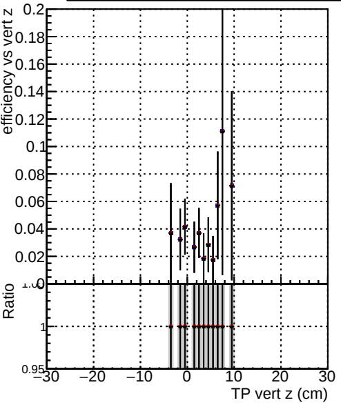
Efficiency vs vertpos DQM_TT_originalREDO100 DQM_TT_originalREDO100f DQM_TT_originalREDO100fb
