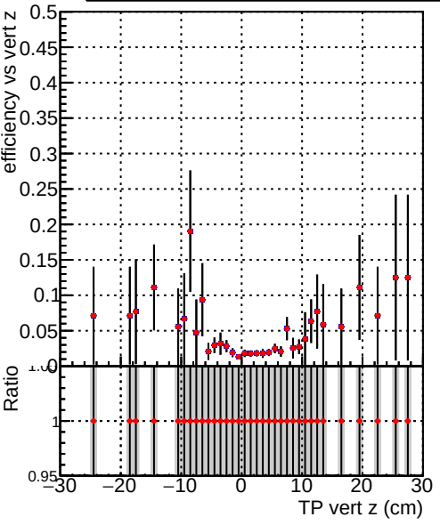
Efficiency vs vert z Legend: DQM_TT_originalREDO100 DQM_TT_originalREDO100f
