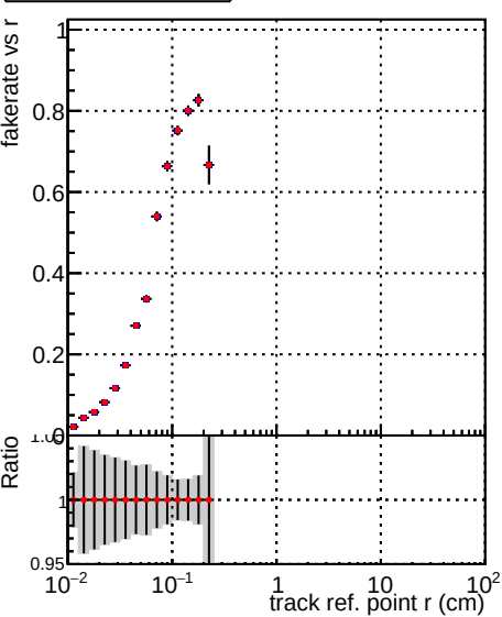
Fake rate vs v —●— DQM_TT_originalREDO100 —●— DQM_TT_originalREDO100f
