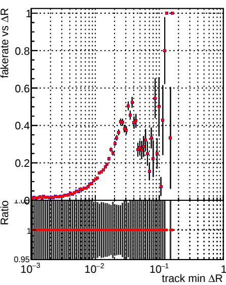
Fake rate vs \Delta R(\text{track, jet}) Legend: \square DQM_TT__originalREDO100 \bullet DQM_TT__originalREDO100f
