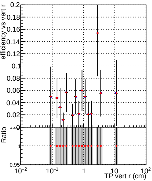
Efficiency vs vertpos Legend: DQM_TT_originalREDO100 DQM_TT_originalREDO100f
