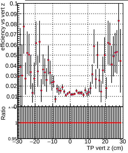
Efficiency vs TP vert z (cm) Legend: — /data2/legianni/pareto-opt/restart/CMSSW_14_0_5/src/MTV-plot/DQM_TT__original_PU — /data2/legianni/pareto-opt/train_area_forExtraParams/CMSSW_14_0_5/src/MTV-plot/DQM_TT__originalREDO
