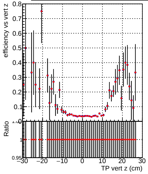
Efficiency vs. TP vert z (cm) for two different simulation setups
