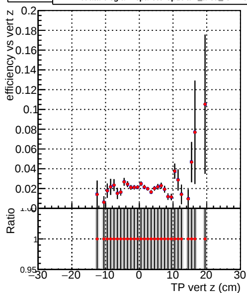
— /data2/legianni/pareto-opt/restart/CMSSW_14_0_5/src/MTV-plot/DQM_TT_original_PU — /data2/legianni/pareto-opt/train_area_forExtraParams/CMSSW_14_0_5/src/MTV-plot/DQM_TT_originalREDO
