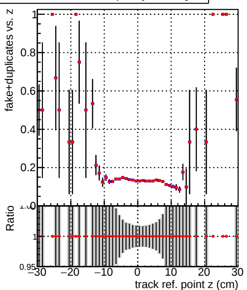
—•— /data2/legianni/pareto-opt/restart/CMSSW_14_0_5/src/MTV-plot/DQM_TT_original_PU —•— /data2/legianni/pareto-opt/train_area_forExtraParams/CMSSW_14_0_5/src/MTV-plot/DQM_TT_originalREDO
