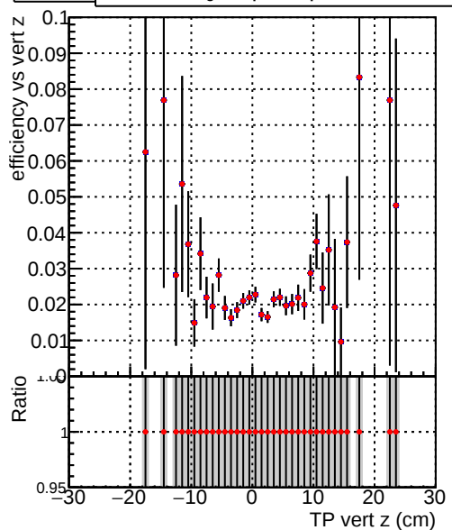
—•— /data2/legianni/pareto-opt/restart/CMSSW_14_0_5/src/MTV-plot/DQM_TT_original_PU —•— /data2/legianni/pareto-opt/train_area_forExtraParams/CMSSW_14_0_5/src/MTV-plot/DQM_TT_originalREDO
