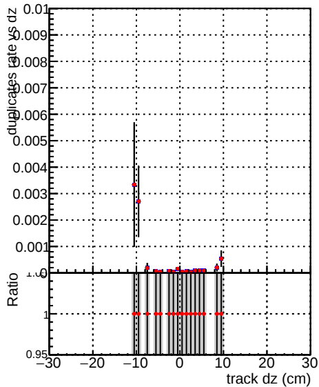
—•— /data2/legianni/pareto-opt/restart/CMSSW_14_0_5/src/MTV-plot/DQM_TT_original_PU —•— /data2/legianni/pareto-opt/train_area_forExtraParams/CMSSW_14_0_5/src/MTV-plot/DQM_TT_originalREDO
