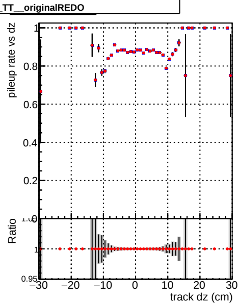
—•— /data2/legianni/pareto-opt/restart/CMSSW_14_0_5/src/MTV-plot/DQM_TT_original_PU —•— /data2/legianni/pareto-opt/train_area_forExtraParams/CMSSW_14_0_5/src/MTV-plot/DQM_TT_originalREDO
