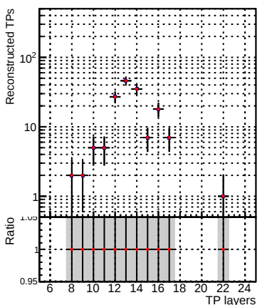
ams/CMSSW_14_0_5/src/MTV-plot/DQM_TT__or
