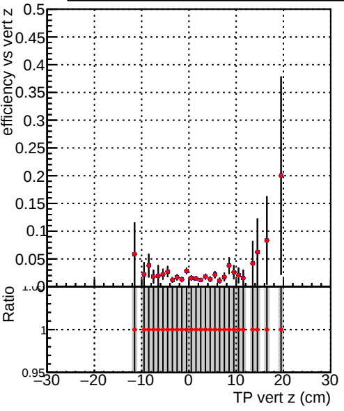
Efficiency vs vert z Legend: — /data2/legianni/pareto-opt/restart/CMSSW_14_0_5/src/MTV-plot/DQM_TT__original_PU — /data2/legianni/pareto-opt/train_area_forExtraParams/CMSSW_14_0_5/src/MTV-plot/DQM_TT__originalREDO
