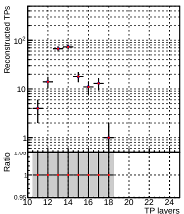
ams/CMSSW_14_0_5/src/MTV-plot/DQM_TT__originalREDO
