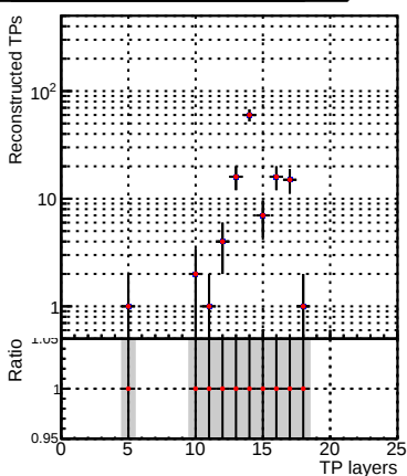
ams/CMSSW_14_0_5/src/MTV-plot/DQM_TT__ori
