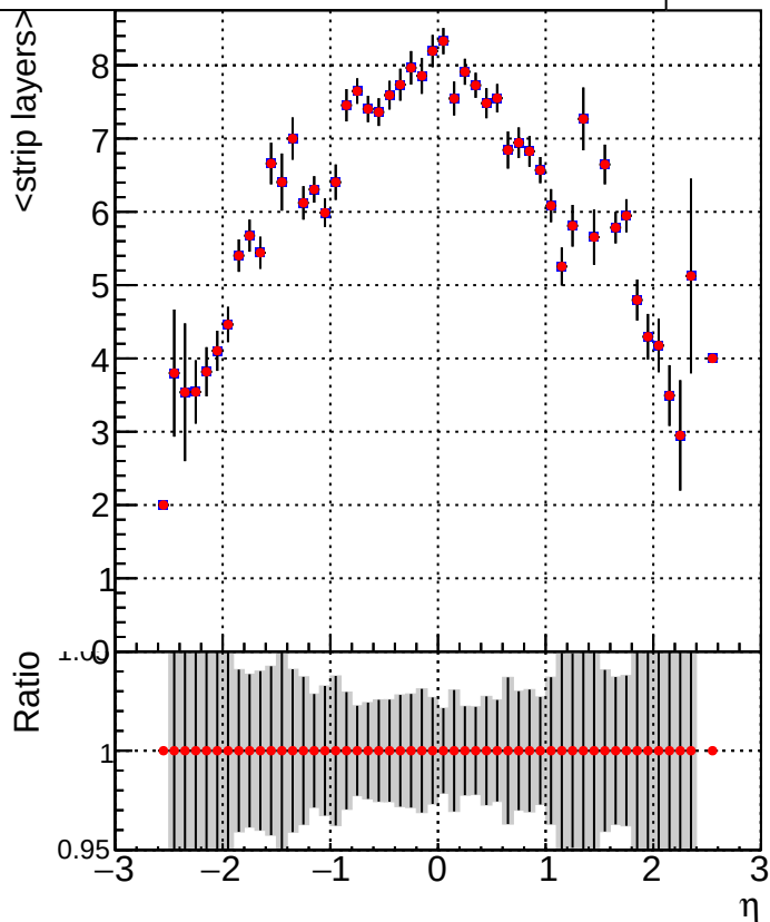
■ /data2/legianni/pareto-opt/restart/CMSSW_14_0_5/src/MTV-plot/DQM_TT_original_PU — /data2/legianni/pareto-opt/train_area_forExtraParams/CMSSW_14_0_5/src/MTV-plot/DQM_TT_originalRE
