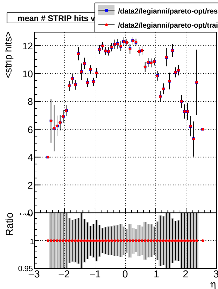
■ /data2/legianni/pareto-opt/restart/CMSSW_14_0_5/src/MTV-plot/DQM_TT_original_PU — /data2/legianni/pareto-opt/train_area_forExtraParams/CMSSW_14_0_5/src/MTV-plot/DQM_TT_originalRE
