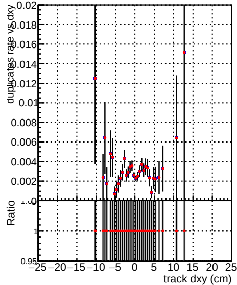
— /data2/legianni/pareto-opt/restart/CMSSW_14_0_5/src/MTV-plot/BQM_TT_original_PU — /data2/legianni/pareto-opt/train_area_forExtraParams/CMSSW_14_0_5/src/MTV-plot/BQM_TT_originalREDO
