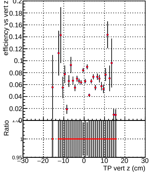
Efficiency vs. TP vert z (cm) for two datasets
