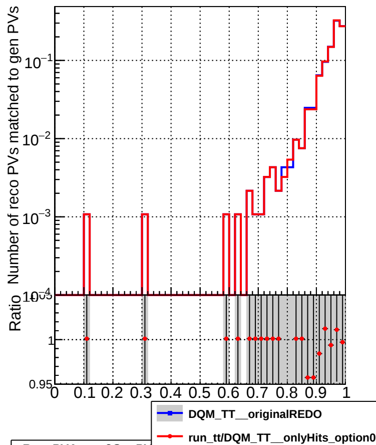
RecoPVAssoc2GenPVmatched_missing
