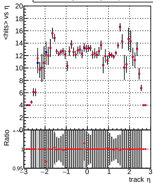
mean hit — DQM_TT__originalREDO — run_tt/DQM_TT__onlyHits_option0
