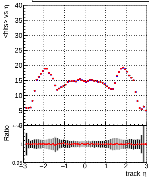
mean hit — DQM_TT__originalREDO — run_tt/DQM_TT__onlyHits_option0
