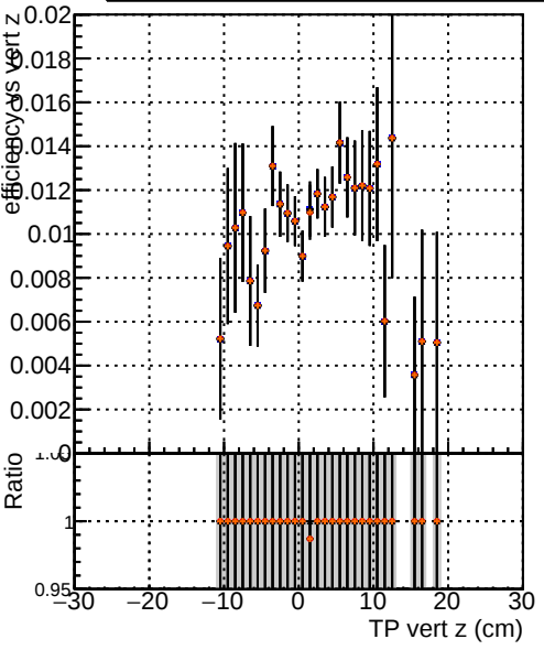
Efficiency vs vertpos — /data2/legianni/pareto-opt/restart/CMSSW_14_0_5/src/MIV-plot/DQM_TT_original_PU — DQM_TT_trainAll2_PU — DQM_TT_trainAll2pth_PU — DQM_TT_trainAll2ptl_PU
