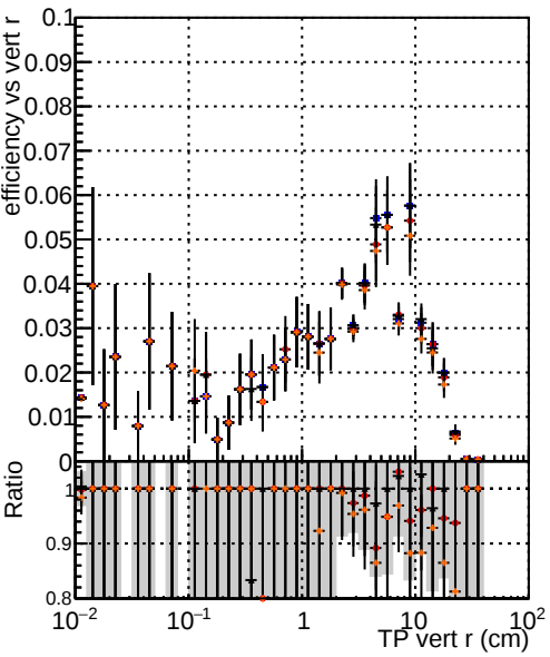
Efficiency vs TP vert r (cm) — /data2/legianni/pareto-opt/restart/CMSSW_14_0_5/src/MTV-plot/DQM_TT_original_PU — DQM_TT_trainAll2_PU — DQM_TT_trainAll2pth_PU — DQM_TT_trainAll2ptl_PU
