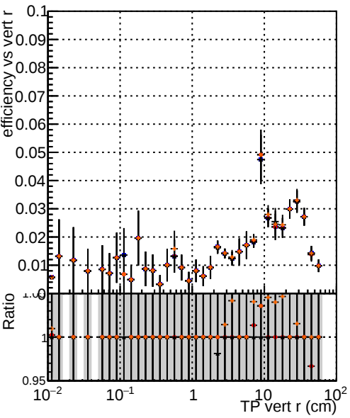
Efficiency vs vertpos — data2/legianni/pareto-opt/restart/CMSSW_14_0_5/src/MTV-plot/DQM_TT_original_PU — DQM_TT_trainAll2_PU — DQM_TT_trainAll2pth_PU — DQM_TT_trainAll2ptl_PU
