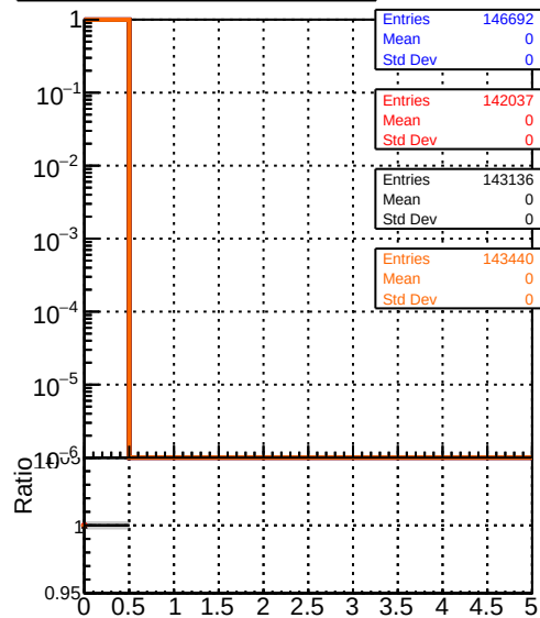
/data2/legianni/pareto-opt/restart/CMSSW_14_0_5/src/MIV-plot/DQM_TT_original_PU mean hits
