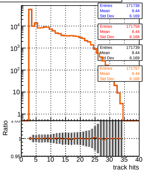
/data2/legianni/pareto-opt/restart/CMSSW_14_0_5/src/MIV-plot/DQM_TT_original_PU DQM_TT_trainAll2_PU DQM_TT_trainAll2pth_PU DQM_TT_trainAll2ptl_PU
