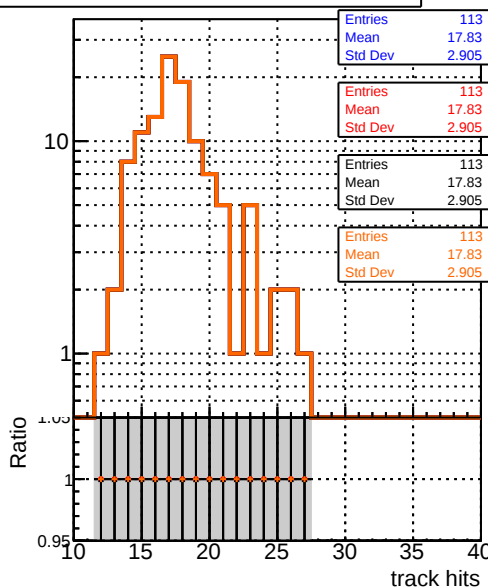
/data2/legianni/pareto-opt/restart/CMSSW_14_0_5/src/MIV-plot/DQM_TT_original_PU DQM_TT_trainAll2_PU DQM_TT_trainAll2pth_PU DQM_TT_trainAll2ptl_PU
