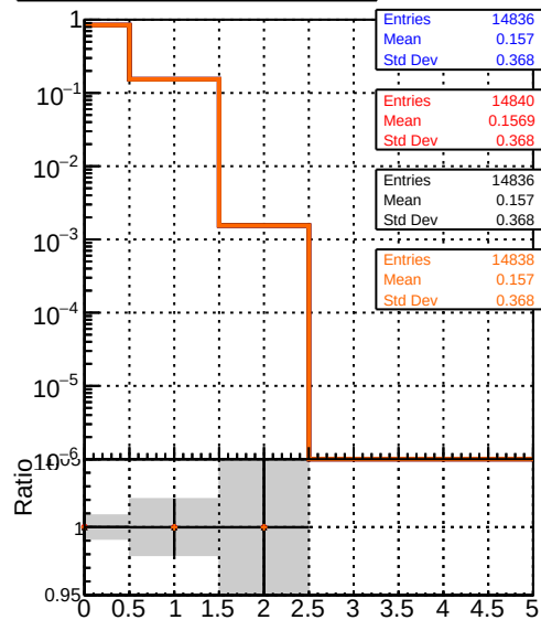
mean hits /data2/legianni/pareto-opt/restart/CMSSW_14_0_5/src/MIV-plot/DQM_TT_original_PU DQM_TT_trainAll2_PU DQM_TT_trainAll2pth_PU DQM_TT_trainAll2ptl_PU
