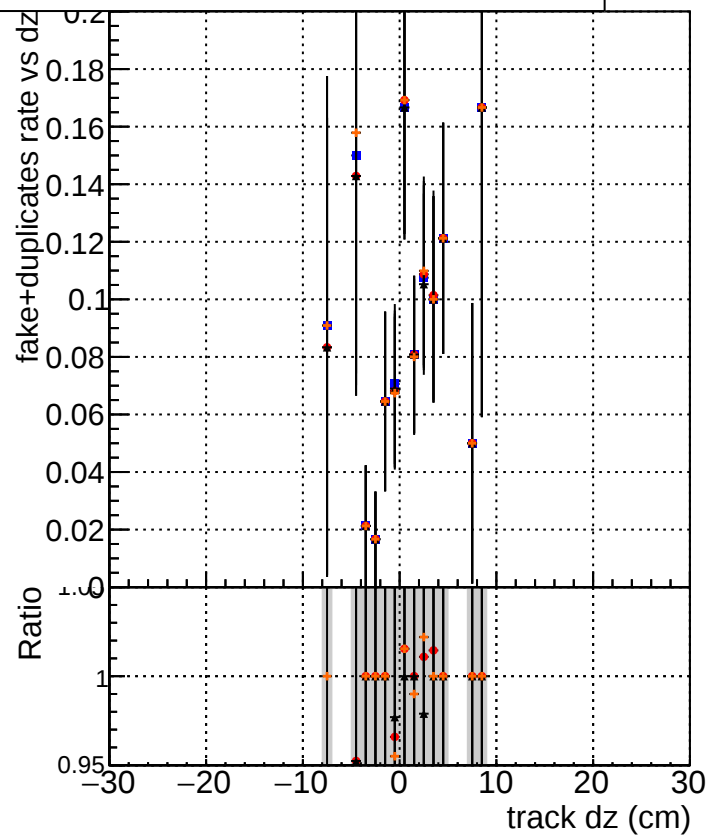
/data2/legianni/pareto-opt/restart/CMSSW_14_0_5/src/MTV-plot/DQM_TT_original_PU DQM_TT_trainAll2_PU DQM_TT_trainAll2pth_PU DQM_TT_trainAll2ptl_PU
