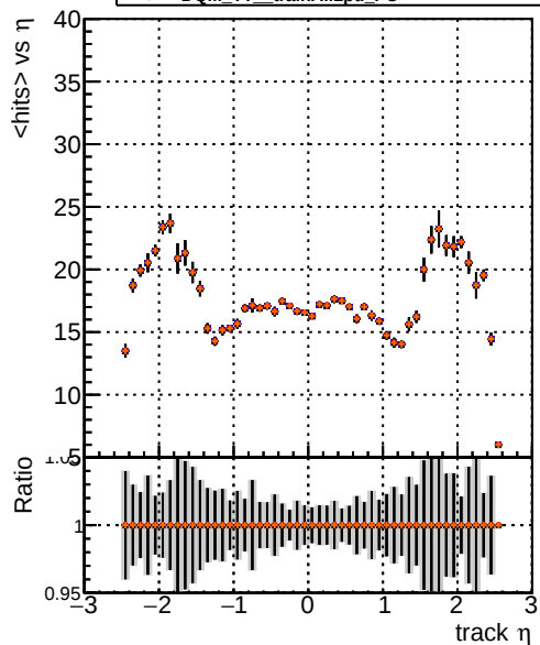
mean hit /data2/legianni/pareto-opt/restart/CMSSW_14_0_5/src/MIV-plot/DQM_TT_original_PU DQM_TT_trainAll2_PU DQM_TT_trainAll2pth_PU DQM_TT_trainAll2ptl_PU
