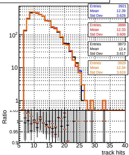
/data2/legianni/pareto-opt/restart/CMSSW_14_0_5/src/MIV-plot/DQM_TT_original_PU DQM_TT_trainAll2_PU DQM_TT_trainAll2pth_PU DQM_TT_trainAll2ptl_PU
