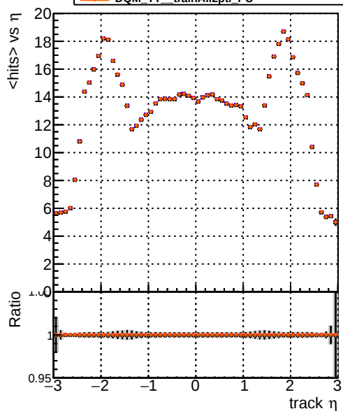
mean hits /data2/legianni/pareto-opt/restart/CMSSW_14_0_5/src/MIV-plot/DQM_TT_original_PU DQM_TT_trainAll2_PU DQM_TT_trainAll2pth_PU DQM_TT_trainAll2ptl_PU
