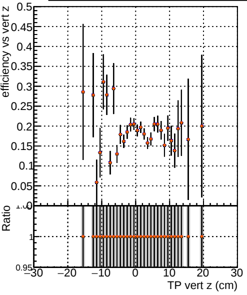
Efficiency vs vertpos Legend: — data2/legianni/pareto-opt/restart/CMSSW_14_0_5/src/MIV-plot/DQM_TT_original_PU — DQM_TT_trainAll2_PU — DQM_TT_trainAll2pth_PU — DQM_TT_trainAll2ptl_PU
