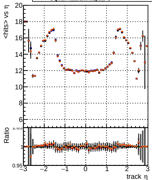
mean hits /data2/legianni/pareto-opt/restart/CMSSW_14_0_5/src/MV-plot/DQM_TT_original_PU DQM_TT_trainAll2_PU DQM_TT_trainAll2pth_PU DQM_TT_trainAll2ptl_PU
