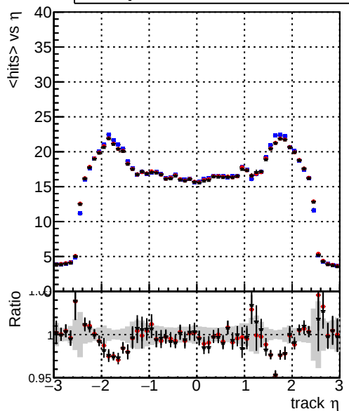
mean hits vs \eta — DQM_TT_original — DQM_TT_modified_models9 — DQM_TT_mod_modelW29
