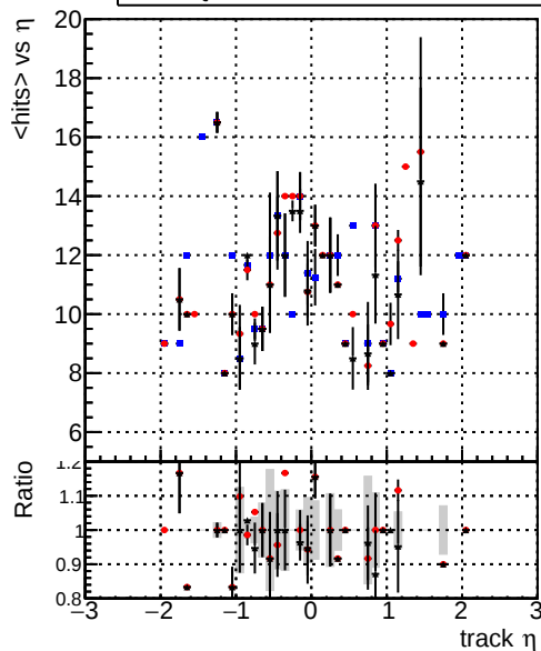
mean hit — DQM_TT_original — DQM_TT_modified_models9 — DQM_TT_mod_modelW29
