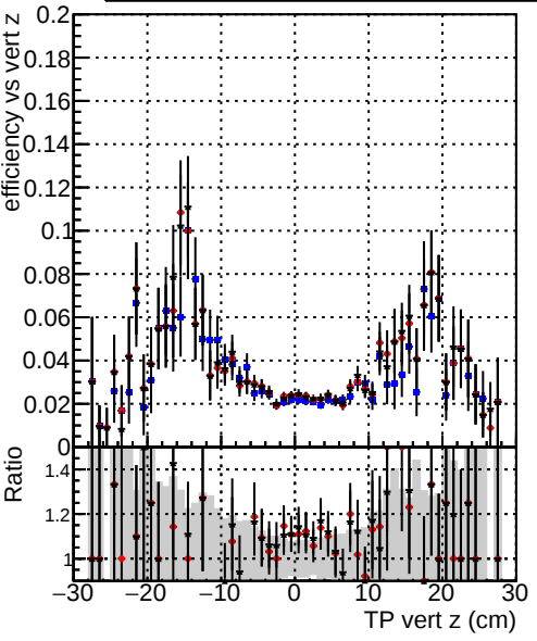
Efficiency vs TP vert z (cm) Legend: DQM_TT_original DQM_TT_modified_models9 DQM_TT_mod_reproduceerror
