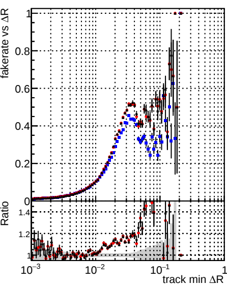
Fake rate vs \Delta R (track, jet) Legend: DQM TT original (black line with blue dots), DQM TT modified models9 (red line with red dots), DQM TT mod_reproduceerror (black line with black dots)
