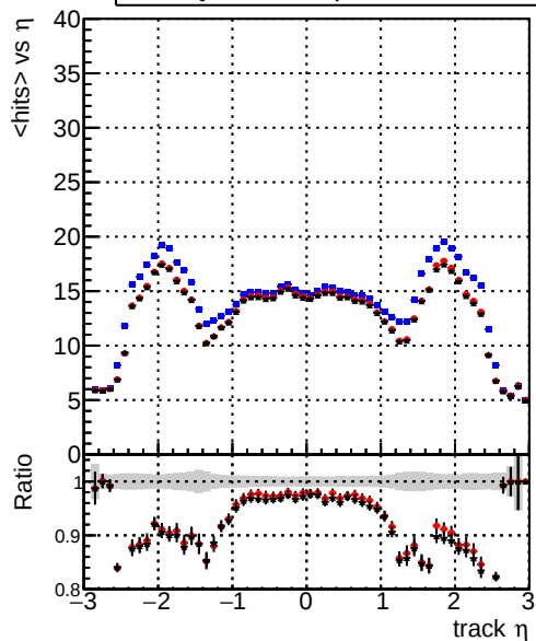
mean hits — DQM_TT_original — DQM_TT_modified_models9 — DQM_TT_mod_reproduceerror
