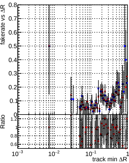
Fake rate vs ΔR(track, jet) Legend: DQM TT original (black line) DQM TT modified models9 (red line) DQM TT mod reproduceerror (blue line)
