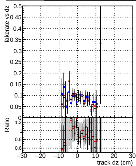
Fake rate vs d DOM TT original DOM TT modified models9 DOM TT mod reproduceerror
