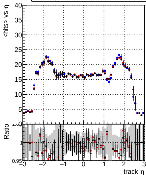
mean hit — DQM_TT_original — DQM_TT_modified_models9 — DQM_TT_mod_reproduceerror
