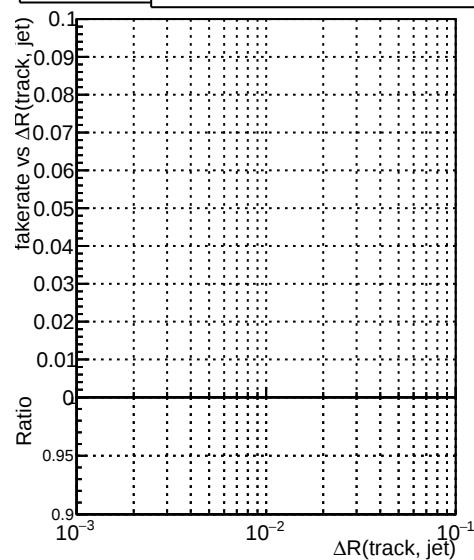
Fake rate vs \Delta R(\text{track, jet}) DQM_V0001_R000000001_Global_CMSSW_X_Y_Z_RECO
