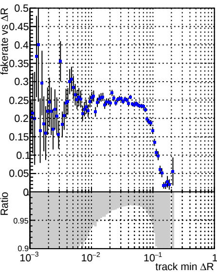
Fake rate vs \Delta R (track, jet) DQM_V0001_R000000001_Global_CMSSW_X_Y_Z_RECO
