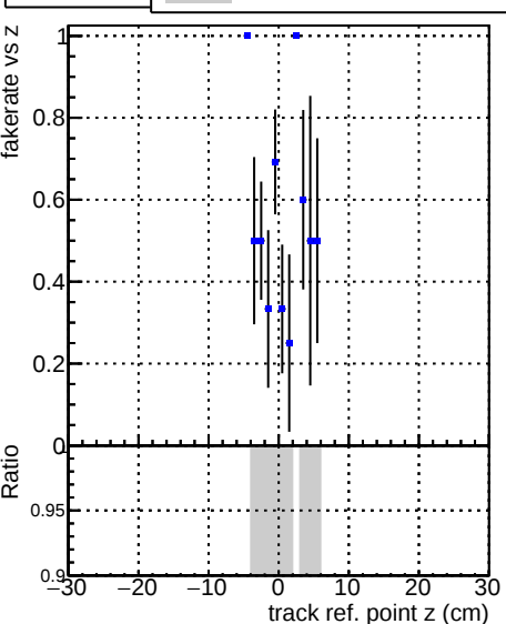
Fake rate vs vertpos DQM_V0001_R000000001_Global_CMSSW_X_Y_Z_RECO
